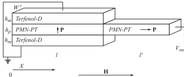
Figure 4. The design of the ME-piezoelectric transformer
