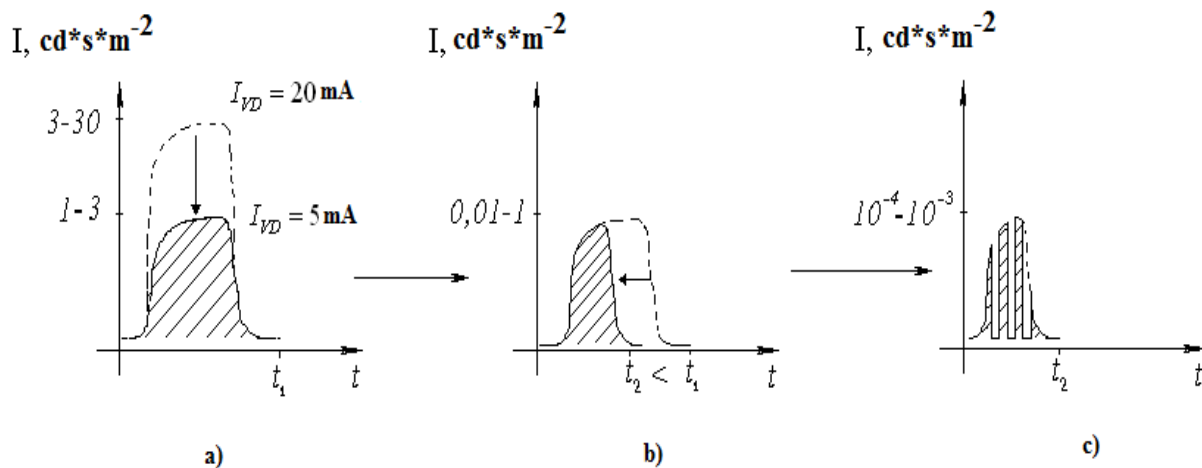
Figure 4. Ways of reducing the intensity of the light stimulus (irritation): a) reducing the electrical power supply parameters of the LED (supply current); b) reducing the duration of the light flash (reducing the exposure); c) using the modulation of the power LED
