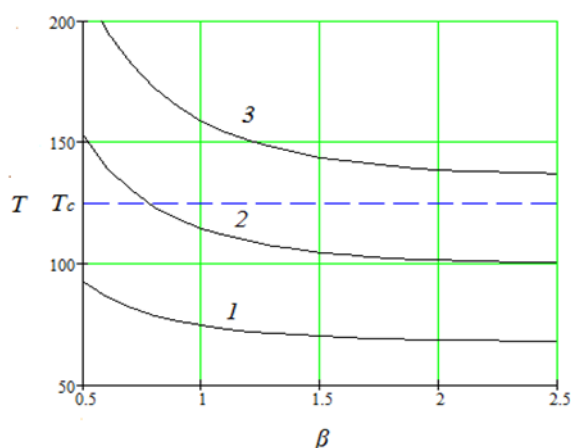
Figure 3. Dependence of the temperature of the active zone of the CMA2550 matrix with a power of P=122 \text{ W} on the reduced length of the HP at the temperature of the medium T_a = 20 \text{ C} and at different heat exchange coefficients. Curve 1 – during forced convection ( \varepsilon=0.1 ), 2 - during free convection ( \varepsilon=0.05 ), 3 – for a solid metal rod of a similar profile during forced convection ( \varepsilon=0.025 )
