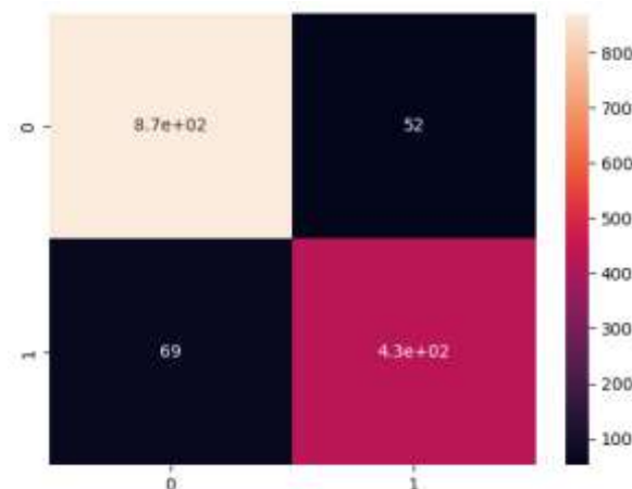
Figure 8. Confusion matrix for improved Random Forest Classifier
