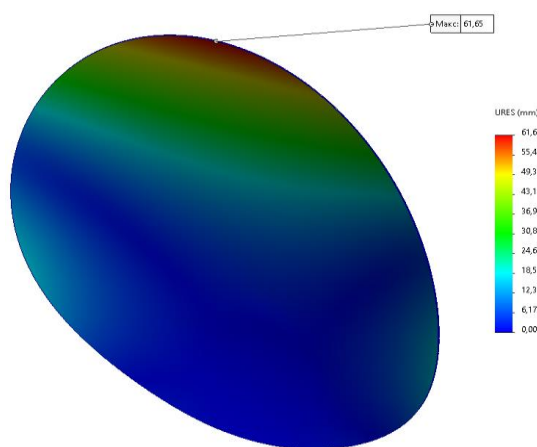
Figure 10. Displacement diagram
