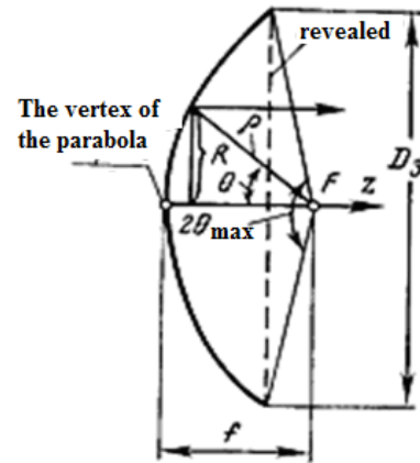
Figure 4. Parabolic antenna opening
