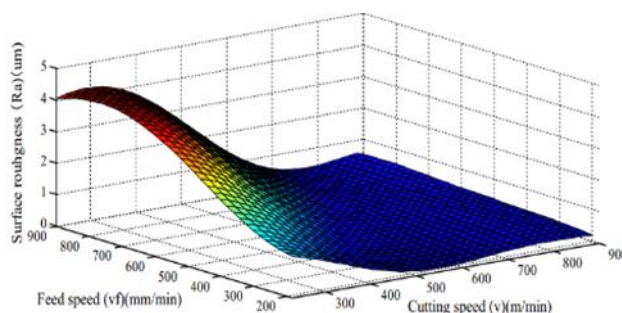
Figure 3. Effect of cutting speed and feedspeed on R_a
