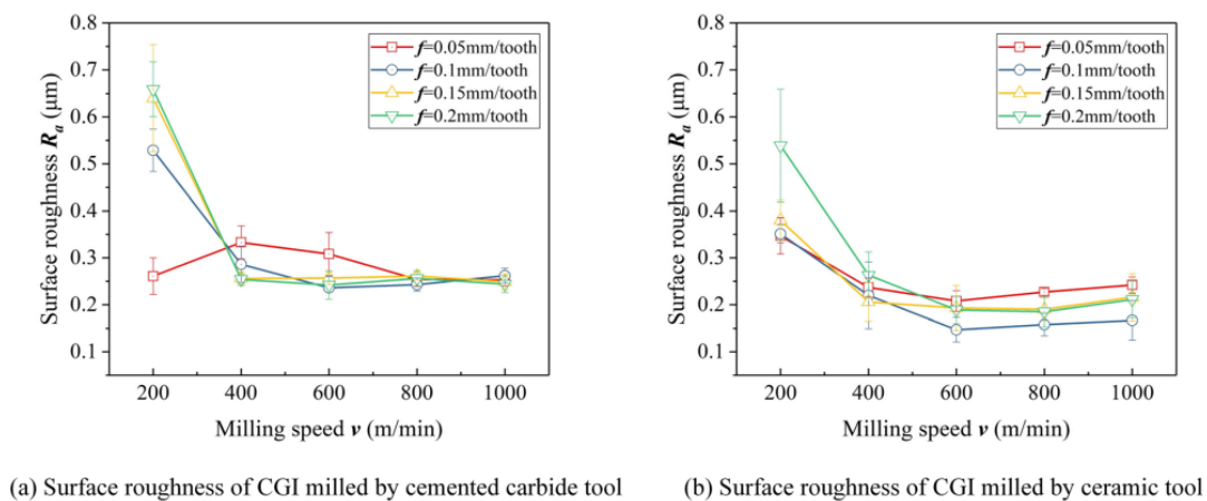
Figure 6. The machined surface roughness of CGI with carbide and ceramic tool.[16]
