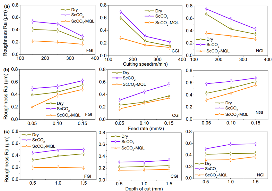
Figure 2. Evolution of machined surface roughness R_a of FGI, CGI, and NGI depend on the (a) cutting speed v_c , (b) feed rate f_z , and (c) depth of cut a_p under dry, \text{ScCO}_2 , and \text{ScCO}_2 -MQL condition [13]
