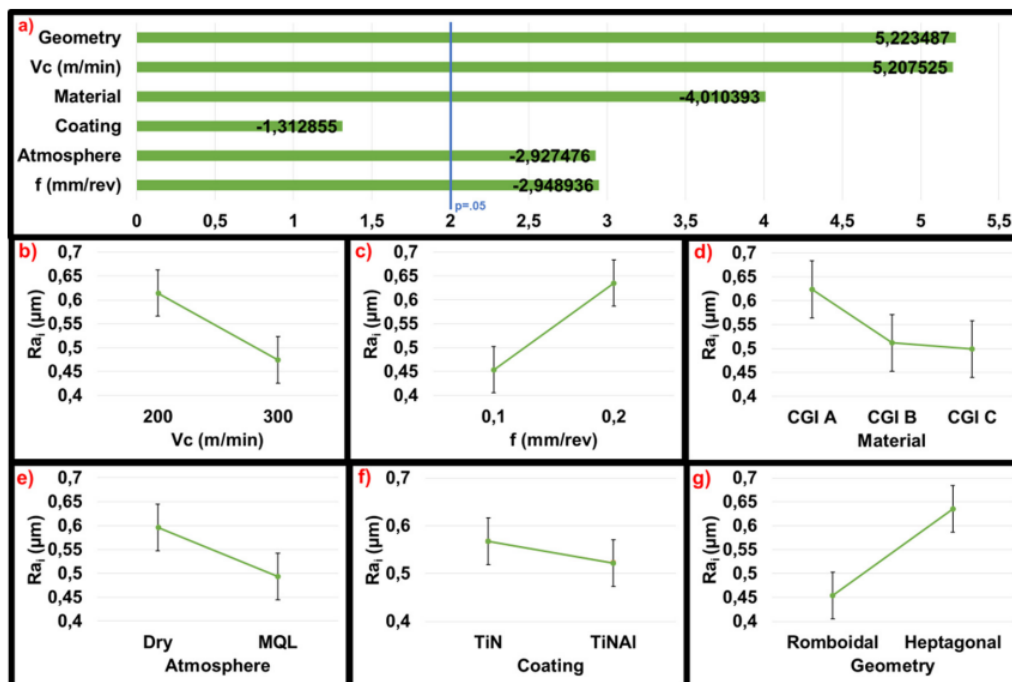
Figure 1. Influence of the input parameters on the roughness of the first machined tool path in the tests. (a) Pareto diagram; (b) influence of the cutting speed; (c) Influence of feed rate; (d) Influence of machined material; (e) Influence of the lubricant condition; (f) influence of the coating; (g) Influence of tool geometry [12]
