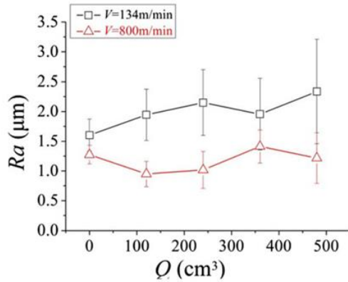
Figure 4. Dependence of roughness and removed material
