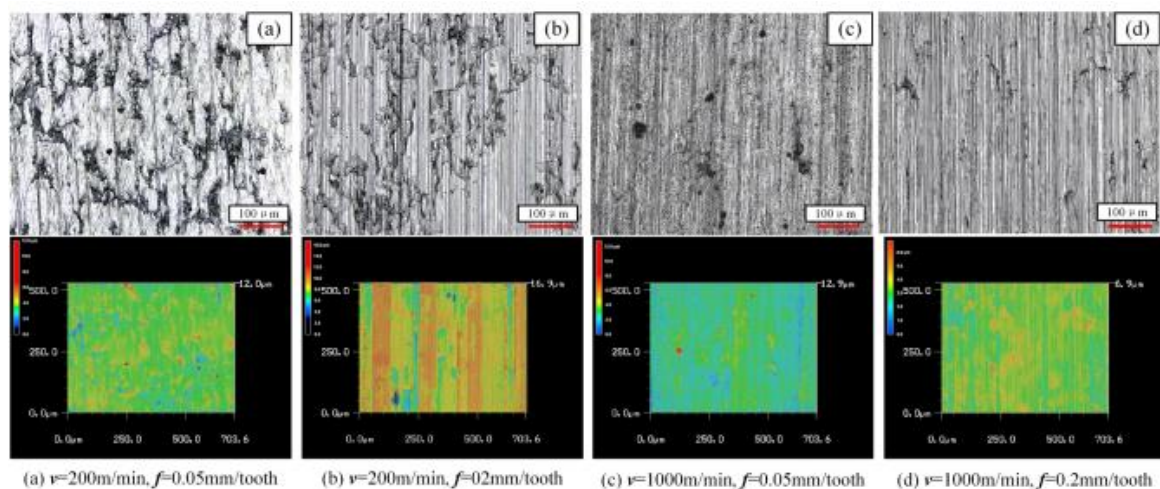
Figure 5. CGI image of the surface after face milling at low 200 m/min and high 1000 m/min cutting speeds [16]
