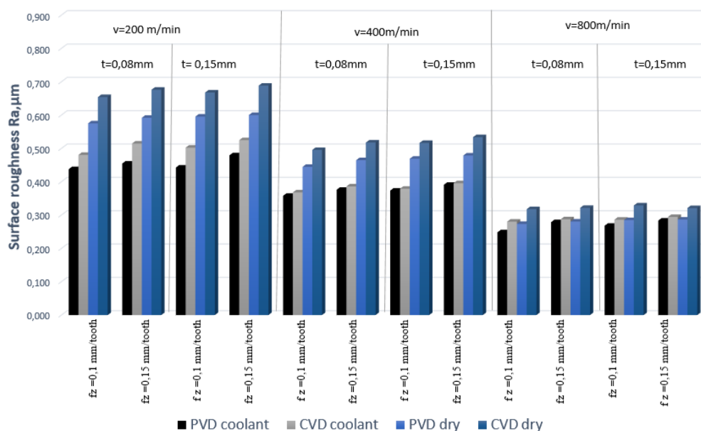
Figure 7. Dependence of various parameters and cutting conditions on surface roughness ( Ra ) when using different types of tools (PVD and CVD) with and without cooling
