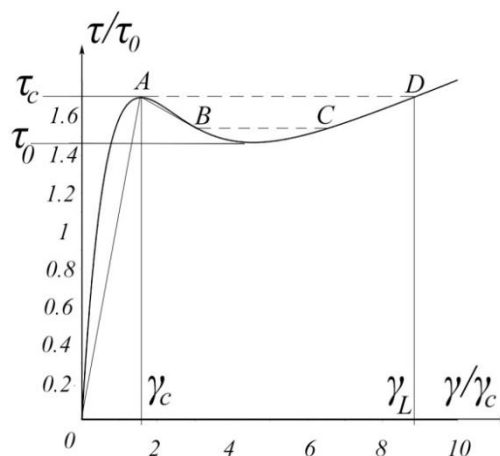
Figure 1. Stress-strain curve \tau \sim \gamma according to equation (1)
