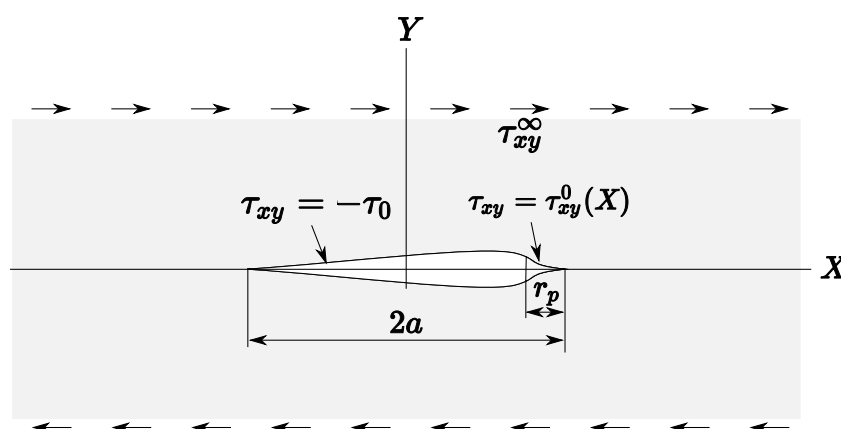
Figure 2. Yoffe problem for mode II crack
