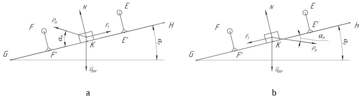
Figure 2. Schemes of the action of forces on the particle when it moves downward – a and upward – b
