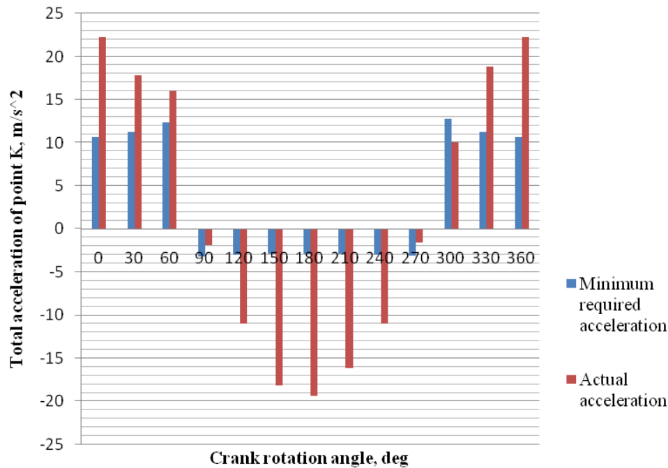
Figure 6. Histogram for comparative analysis of behavior particles at point K
