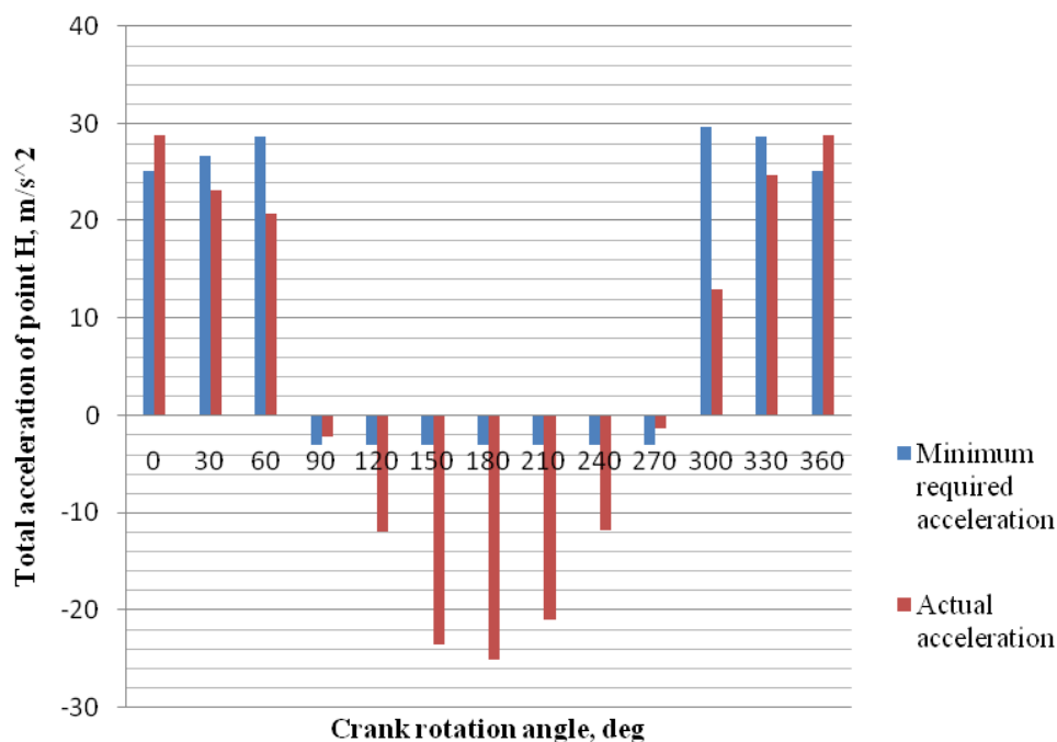
Figure 7. Histogram for comparative analysis of behavior particles at point H
