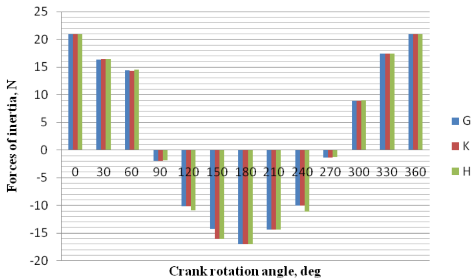
Figure 3. Inertia forces affecting the unit mass at points G, K, H
