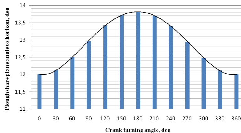
Figure 4. Position of ploughshare plane from crank turning angle
