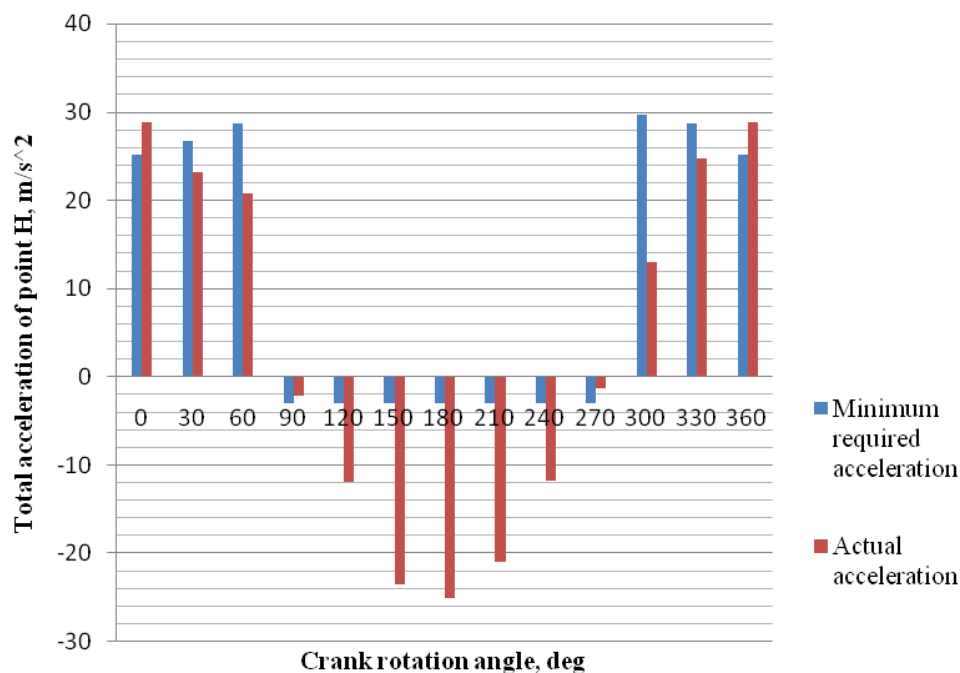
Figure 8. Histogram for comparative analysis of the particle behavior at point H , provided that it is detached from the plane of the ploughshare
