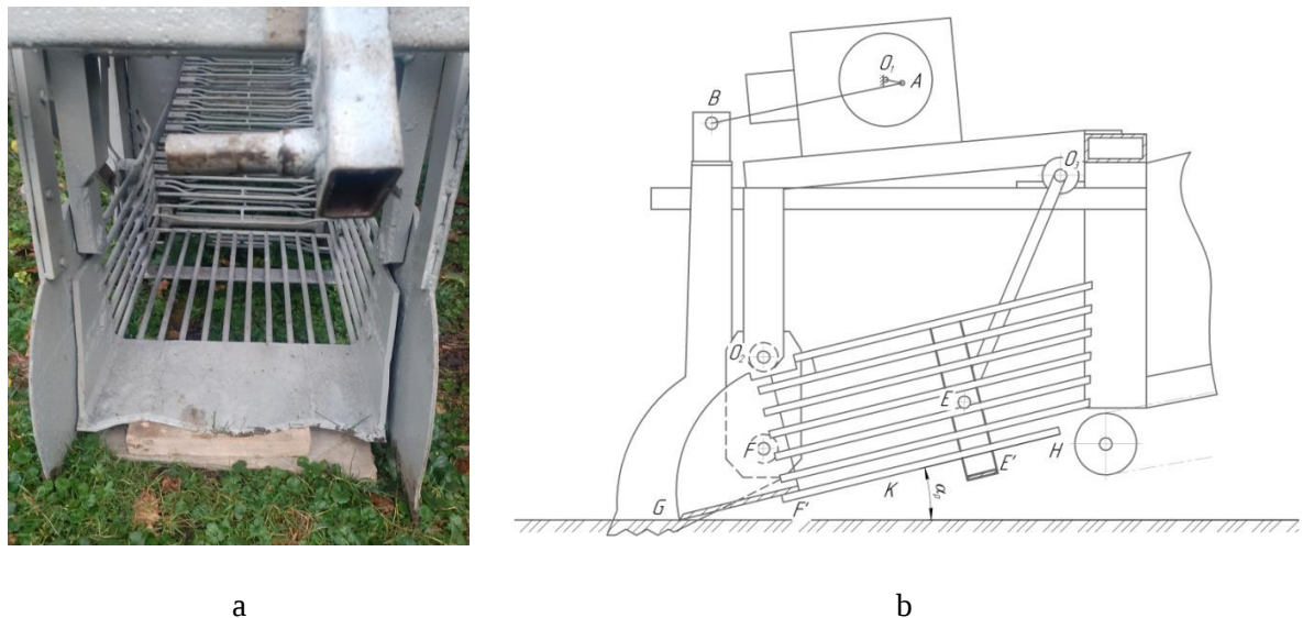
Figure 1. General view of the ploughshare of potato digger – a; its scheme – b
