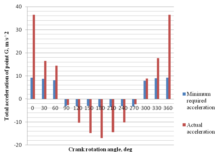
Figure 5. Histogram for comparative analysis of behavior particles at point G
