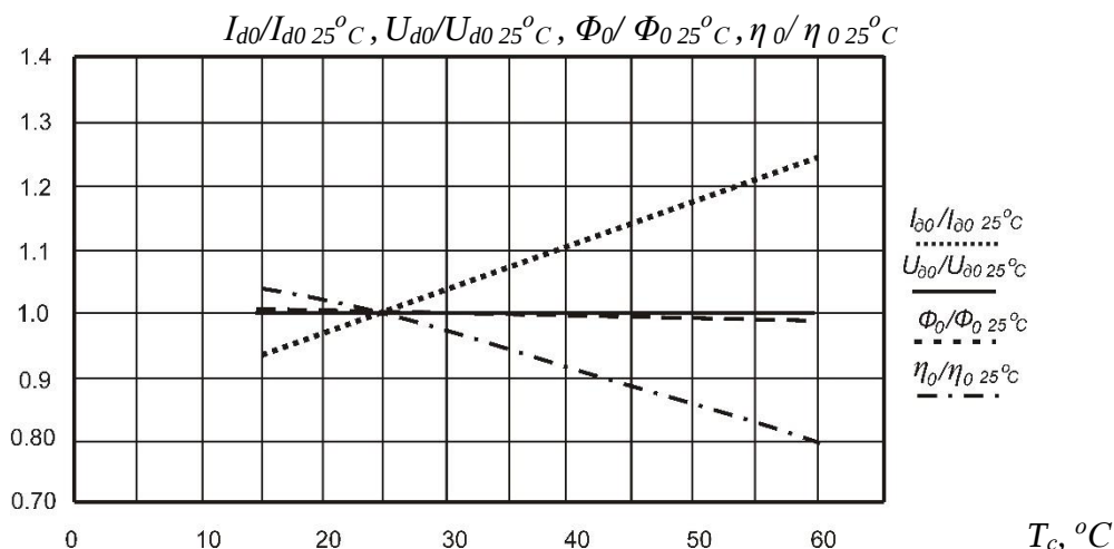
Figure 4. Dependencies I_{d0}/I_{d0\ 25^\circ\text{C}} , U_{d0}/U_{d0\ 25^\circ\text{C}} , \Phi_0/\Phi_0\ 25^\circ\text{C} and \eta_0/\eta_0\ 25^\circ\text{C} on temperature T_c for smd2835 LED. U_{d0\ 25^\circ\text{C}}=18,5\text{B}=\text{const}
