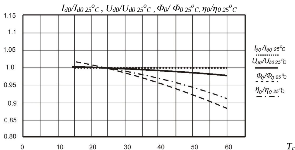
Figure 8. Dependencies I_{d0}/I_{d0\ 25^\circ C} , U_{d0}/U_{d0\ 25^\circ C} , \Phi_0/\Phi_{0\ 25^\circ C} and \eta_0/\eta_{0\ 25^\circ C} on temperature T_c for the lamp P=6W . U_{AC}=\text{const}=220\text{ V}
