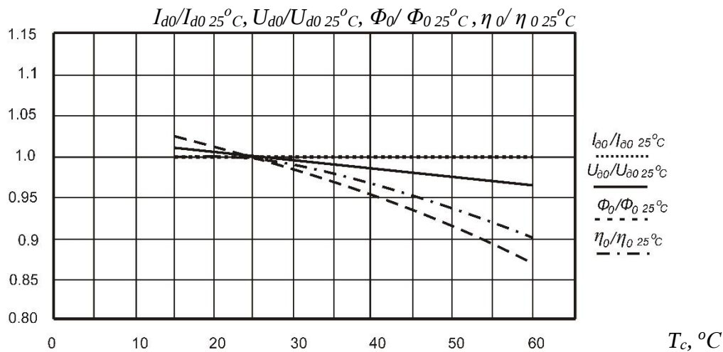
Figure 2. Dependencies I_{d0}/I_{d0\ 25^{\circ}C} , U_{d0}/U_{d0\ 25^{\circ}C} , \Phi_0/\Phi_{0\ 25^{\circ}C} and \eta_0/\eta_{0\ 25^{\circ}C} on the temperature T_c for smd2835 LED. I_{d0\ 25^{\circ}C}=50\text{mA}=\text{const}
