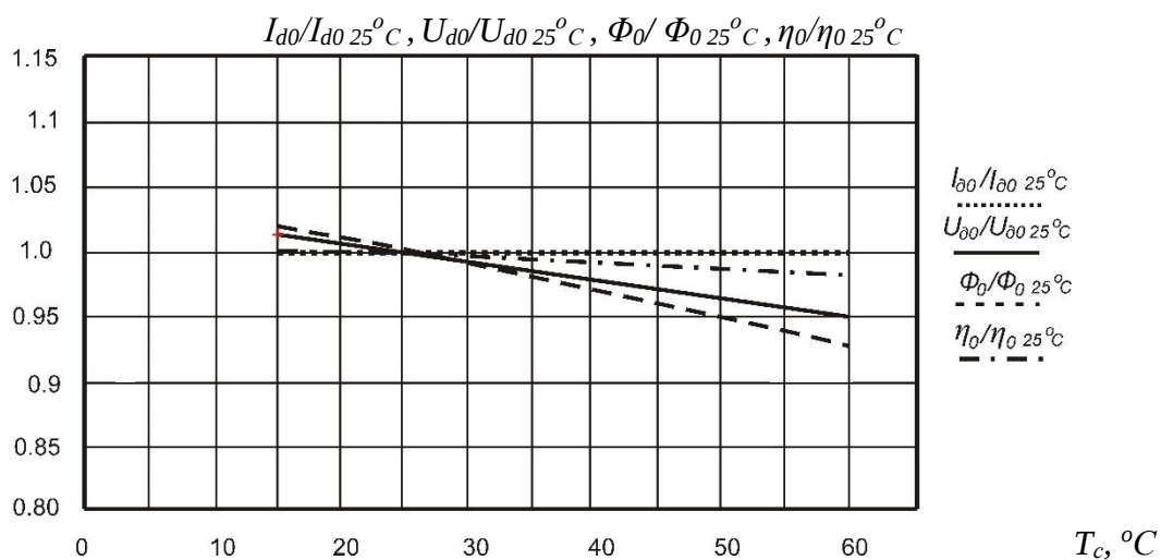
Figure 3. Dependencies I_{d0}/I_{d0\ 25^{\circ}C} , U_{d0}/U_{d0\ 25^{\circ}C} , \Phi_0/\Phi_{0\ 25^{\circ}C} and \eta_0/\eta_{0\ 25^{\circ}C} on temperature T_c for smd5050 LED. I_{d0\ 25^{\circ}C}=60\text{mA}=\text{const}
