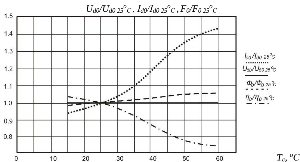
Figure 5. Dependencies I_{d0}/I_{d0\ 25^\circ\text{C}} , U_{d0}/U_{d0\ 25^\circ\text{C}} , \Phi_0/\Phi_0\ 25^\circ\text{C} and \eta_0/\eta_0\ 25^\circ\text{C} on temperature T_c for smd5050 LED. U_{d0\ 25^\circ\text{C}}=3,1\text{B}=\text{const}
