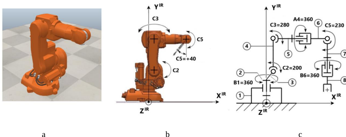
Figure 1. Virtual model of the ABB IRB 140 IR: general view (a), side projection (b) and coordinate system taking into account the attached gripper (tool), frame (thread) model (c) of the kinematic structure of the IR
