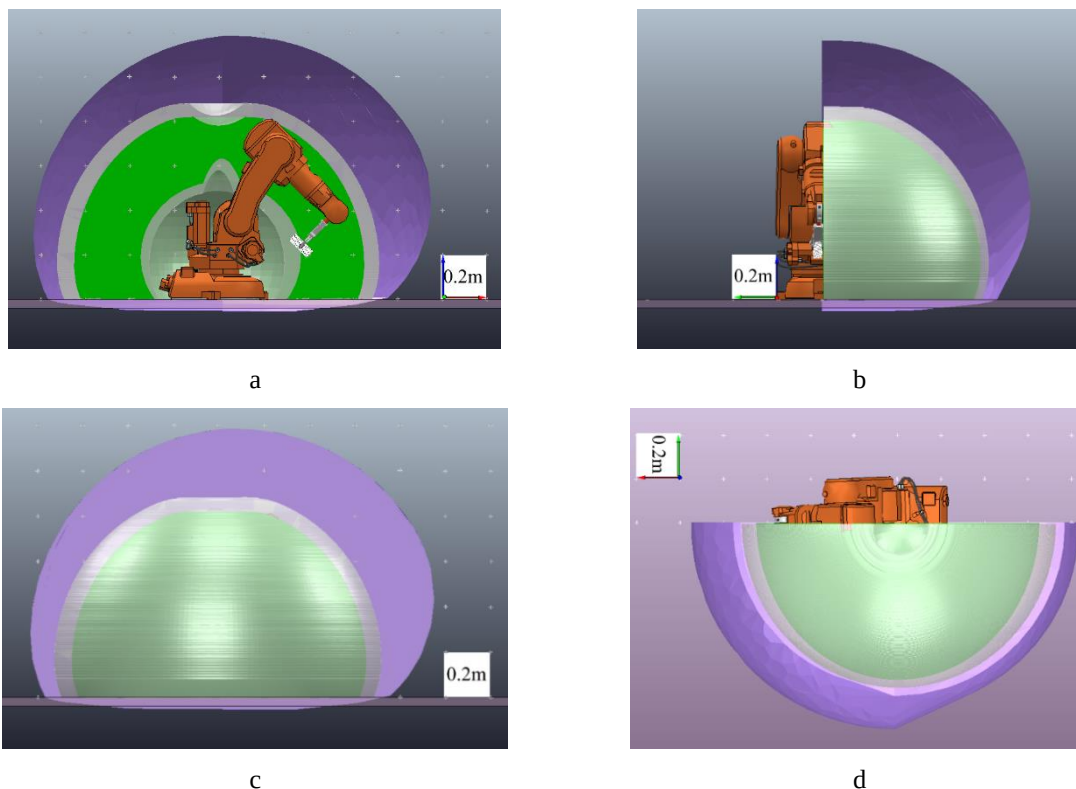
Figure 5. Interface with multiple projections (a, b, c, d), displaying the results of modelling the operating areas of the IR taking into account the angular position of the IR grip (the following elements are presented in different colors: purple – the area of maximum reach of the grip center without taking into account the fixed angular position of the IR grip; green – the working zone taking into account the collision-free reach of the grip center and the fixed angular position of the IR grip; gray – the operating area taking into account the collision-free spatial placement of the workpiece that is in the IR grip, which (the grip) is in the fixed angular position)
