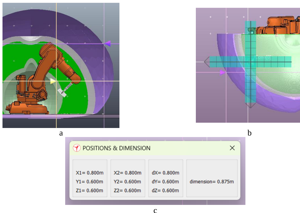
Figure 7. Measuring movable indicators of the dimensions of operating areas: selected positions of the size indicators (projection: side view) (a); visualization of the axes of movement of the indicators (projection: top view) (b); interface window displaying the current measured coordinates of the centers of the indicator axes and the value of the calculated size (c)
