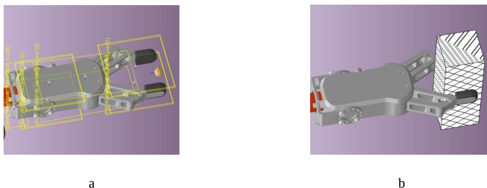
Figure 2. Virtual model of the RG 2 IR gripper: general view (a) taking into account the array of collision control planes; general view (b) taking into account the location of the workpiece in the gripper
