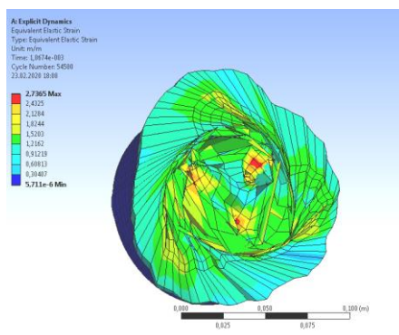
Figure 10. Formation of a whole during rock destruction by the solid drill bit (Ansys WorkBench 18,2 screenshot (academician version))
