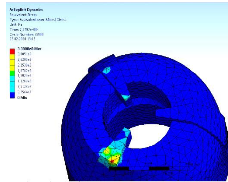
Figure 7. Stresses distribution in the solid drill bit while digging in (Ansys WorkBench 18,2 screenshot (academician version))
