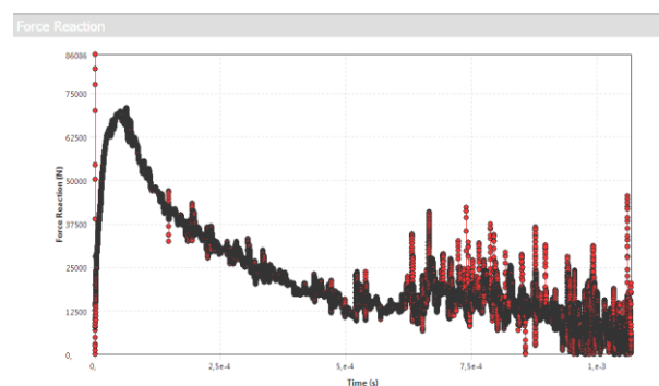
Figure 11. Rock reaction force dynamics during rock destruction by the solid drill bit (Ansys WorkBench 18,2 screenshot (academician version))
