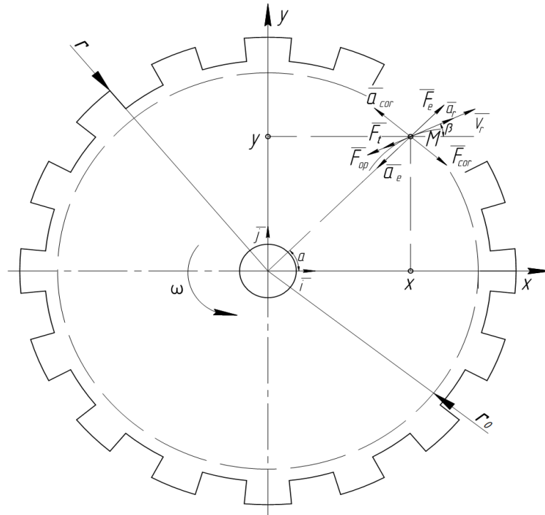
Figure 2. Diagram of the location of a point (molten particle) on the disk and the forces acting on it M – point (molten particle); \vec{F}_t – sliding friction force; \vec{F}_{op} – force of viscous resistance; \vec{F}_e – transfer force of inertia; \vec{F}_{cor} – Coriolis inertia force; \vec{V}_r – relative velocity of the particle; \beta – angle between the vector \vec{V}_r and axis x ; \vec{a}_{cor} – Coriolis acceleration; \vec{a}_e – figurative acceleration; \vec{a}_r – relative acceleration; \omega – angular velocity; \alpha – angle between the radius-vector of the point M and the axis x ; r_0 – distance of the point M from the axis of rotation at the initial moment of time ( r_0 = 0.092\text{ m} ); r – radius of the disk, the position of the point M at the final moment ( r = 0.105\text{ m} )
